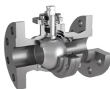
METAL SEATED
