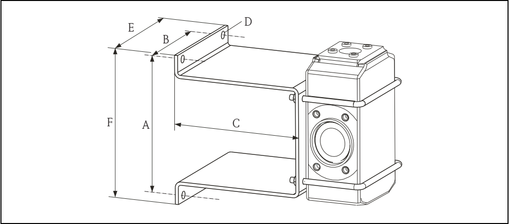
Dimensions in mm (inch)
